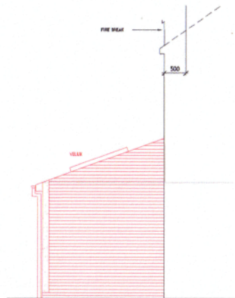
PROPOSED REAR ELEVATION / SECTION 1-50 (LOOKING EAST)
