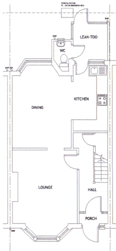
EXISTING GROUND FLOOR PLAN 1-50
