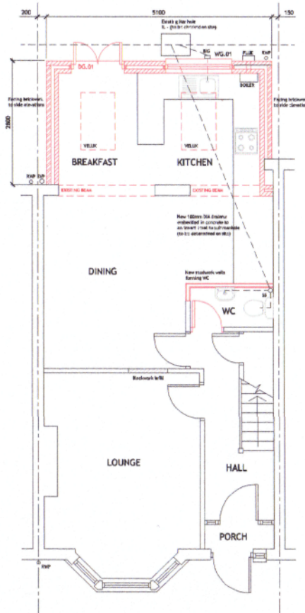
PROPOSED GROUND FLOOR PLAN 1-50
